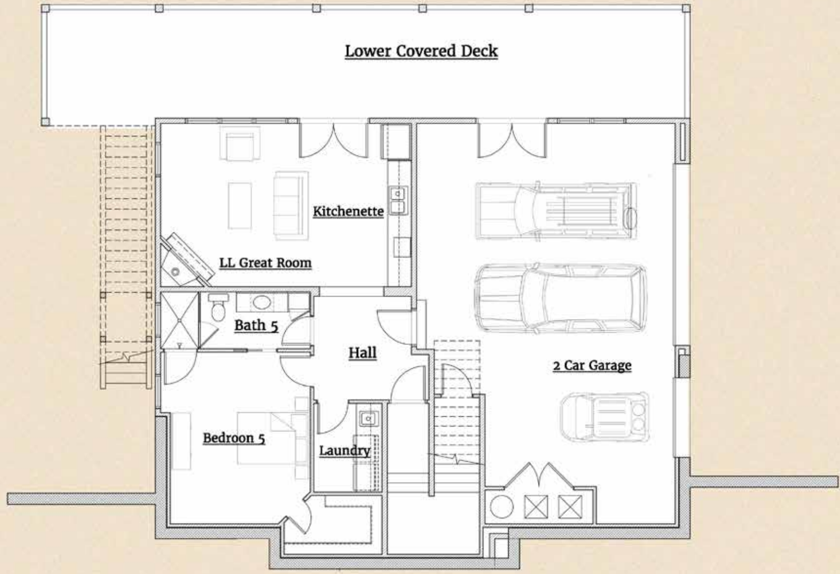
3 SECOND LEVEL FLOOR PLAN
