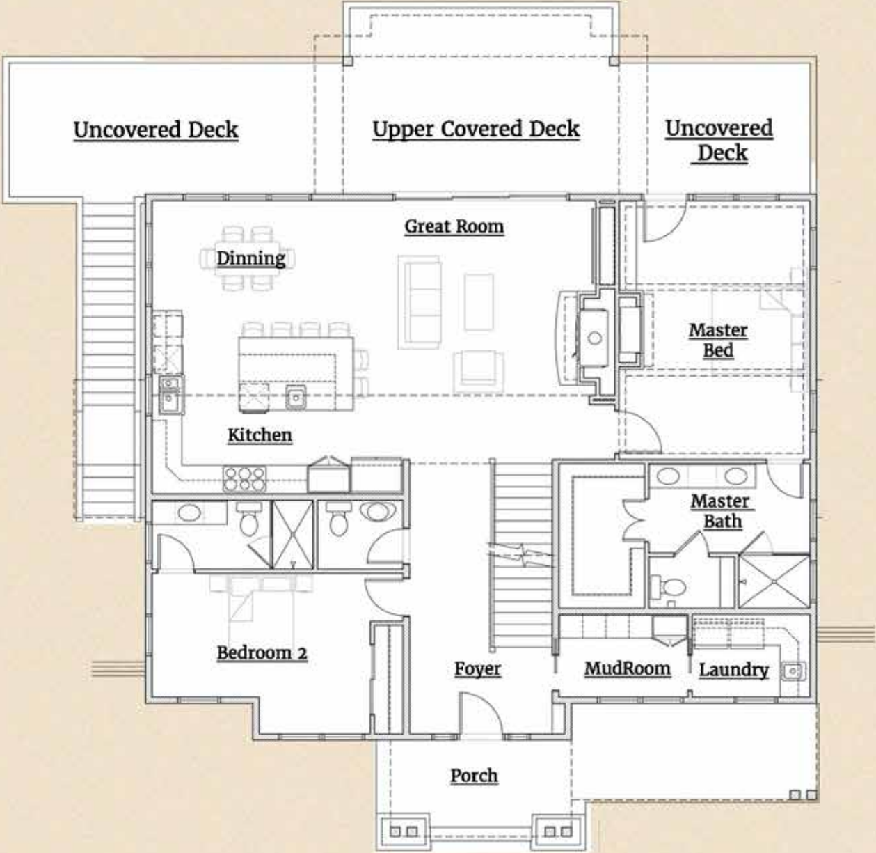
1 MAIN LEVEL FLOOR PLAN
