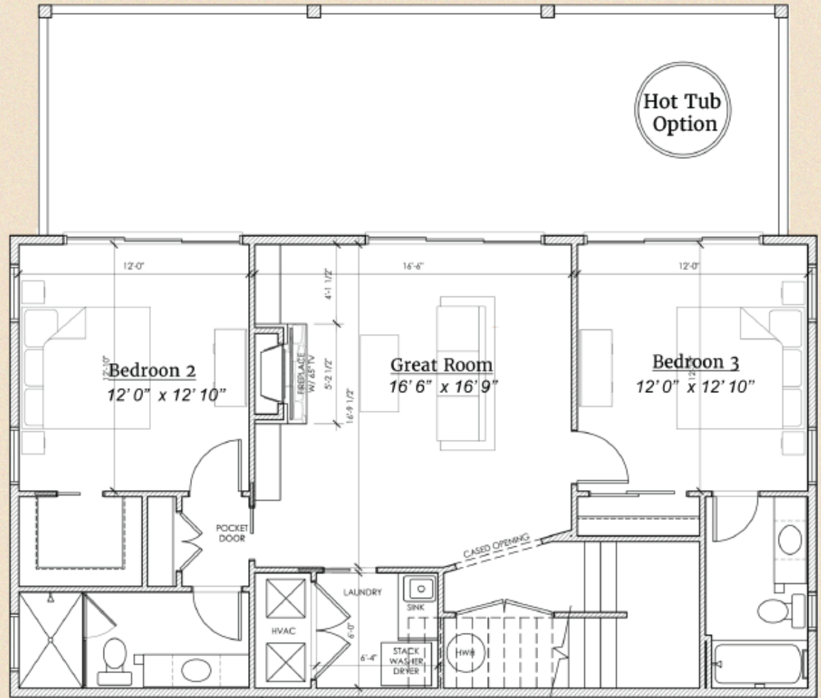
LOWER FLOOR 'B'
